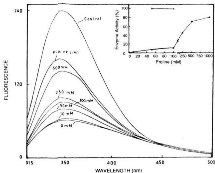
Figure 2C. Fluorescence emission spectra of LDH-M_4 , control (without GuHCl and proline) and GuHCl (0.5 M) denatured enzyme with different concentrations of proline as indicated. The inset shows the enzyme activity in the presence (●) and absence of GuHCl (▲).
