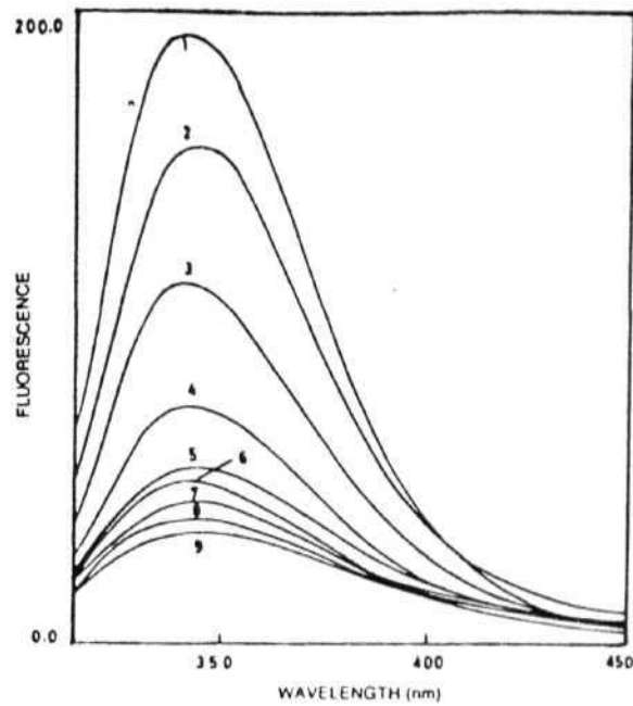
Figure 4.2.1 Fluorescence emission spectra of LDH-M4 (1) control, (2-8) freeze-thawed in the presence of 1.0 M each of (2) proline , (3) sucrose, (4) mannitol , (5) glycine (6) hydroxy proline, (7) glucose, (8) valine and (9) freeze-thawed enzyme.
