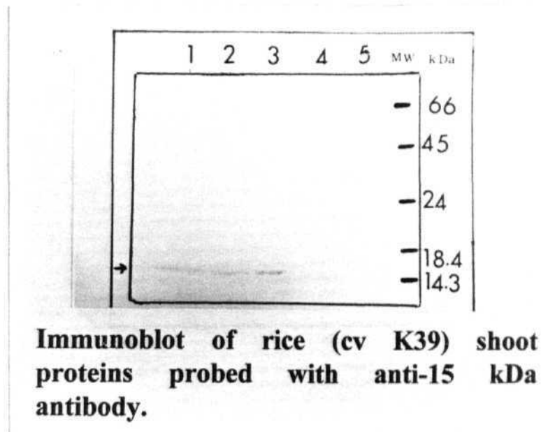
Figure 4.1.6.A. Western analysis of the induction of 15 kDa polypeptide in rice shoots in response to different concentrations of ABA. Lanes (1) 100 \mu\text{M} ABA (2) 60 \mu\text{M} ABA, (3) 20 \mu\text{M} ABA, (4) 10 \mu\text{M} ABA, (5) control. Equal quantity of sample (75 \mu\text{g} ) was loaded into each slot.
