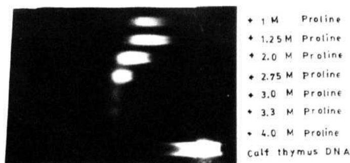
Fig. 4. S1 nuclease sensitivity of calf thymus DNA in the presence of different concentrations of proline.
