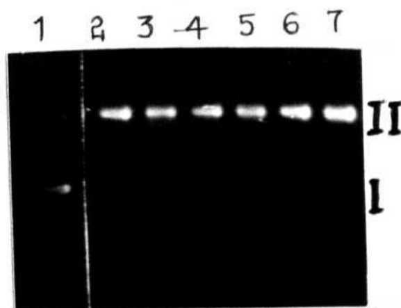
Figure 4.3.13 Topoisomerase I activity on pBR 322 DNA in the presence of increasing concentration of proline and betaine. Lanes (1) pBR 322 plasmid (2) no proline, (3) 2 M proline, (4) 2 M betaine, (5) 3 M proline, (6) 3 M betaine, (7) 5 M proline.
