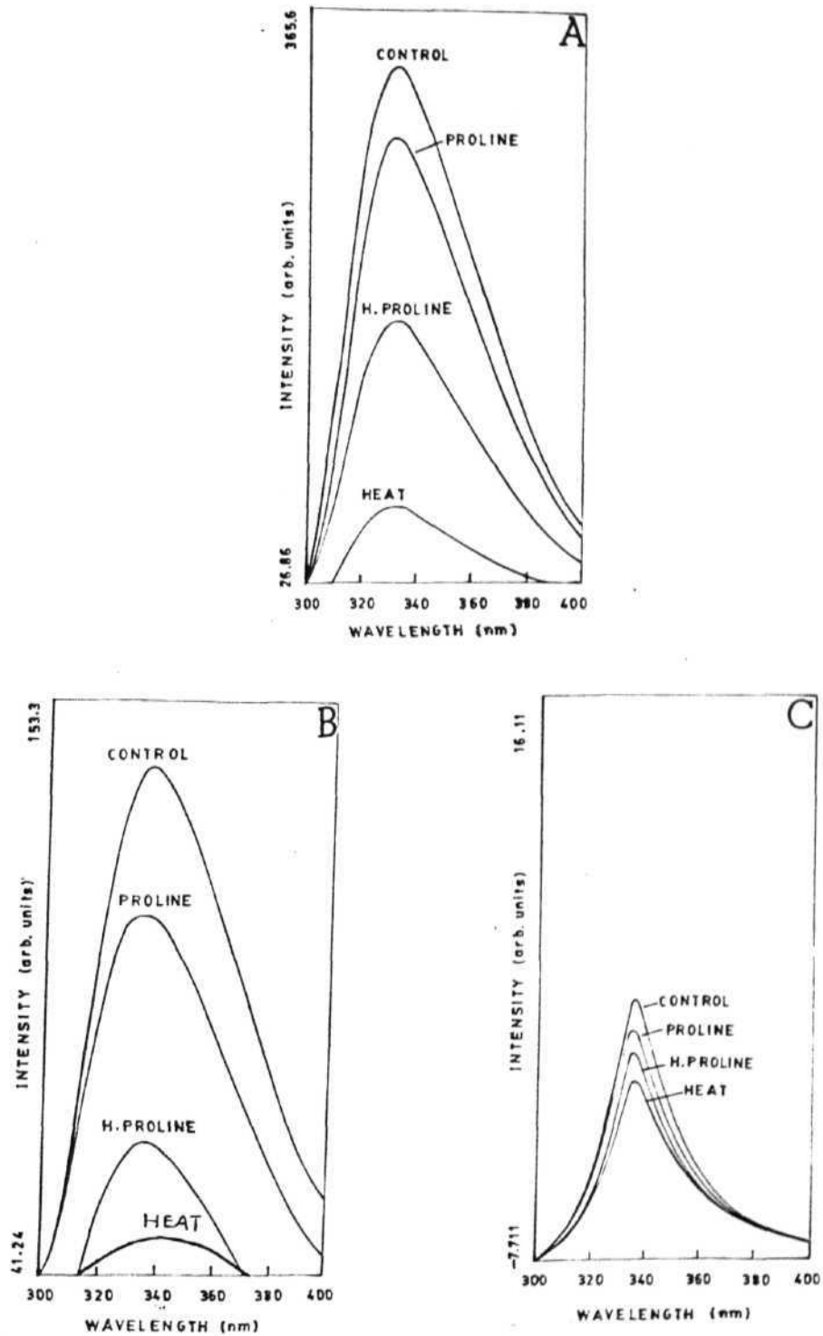
Figure 4.2.13 Fluorescence emission spectra of (A) Eco RV (EC 3.1.21.4) (B) Bara HI (EC 3.1.21.4) and (C) Eco RI (EC 3.1.21.4) heat stressed (50 °C) in the presence of proline and hydroxy proline (1 M).
