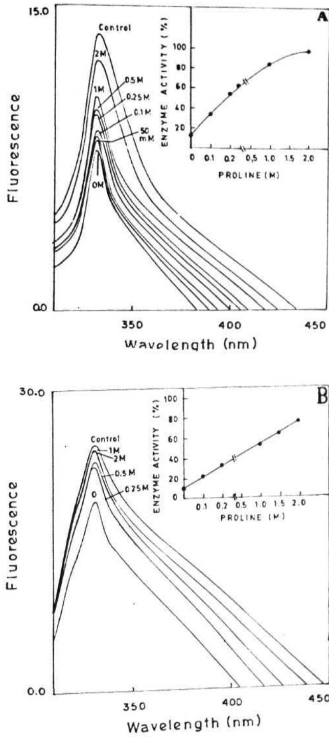
Figure 4.2.8 Fluorescence emission spectra of malate dehydrogenase (EC 1.1.1.37) (A) chemically (GuHCl) denatured (B) heat stressed (50 °C) in the presence of increasing concentration of proline. Insets show the corresponding enzyme activity.
