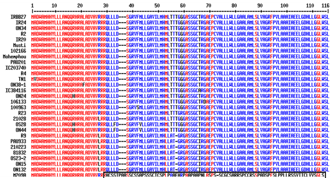
Fig. 4.2.14: Output of multiple alignment for the predicted amino acid sequences of Xa27 alleles. The rice genotypes are indicated in left column. Alignment was performed using Multalin program. The numbers on the top of the sequences indicate the position of amino acids. Insertions and deletions are shown with gaps. Different colors in amino acid shows non synonymous changes. Frameshift mutation in M209A is also shown in the bottom.
