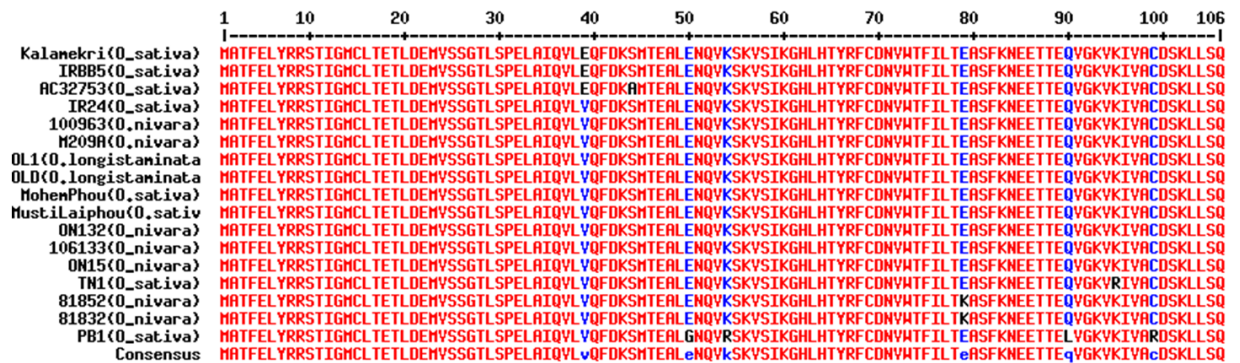
Fig. 4.2.18: (A) Multiple alignment of coding region of xa5 alleles. Substitutions in the CDS are represented with different colors. (B) Output of multiple alignment for the predicted amino acid sequences of xa5 alleles. The rice genotypes are indicated in left column. The numbers on the top of the positions indicate the position of amino acids. Different colors in amino acid shows non synonymous changes. Alignment was performed using Multalin program.
