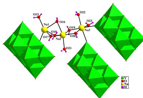
Figure 4.5. The tri-sodium aqua cation coordinated with the three surrounding decavanadate anions in compound 2 .
