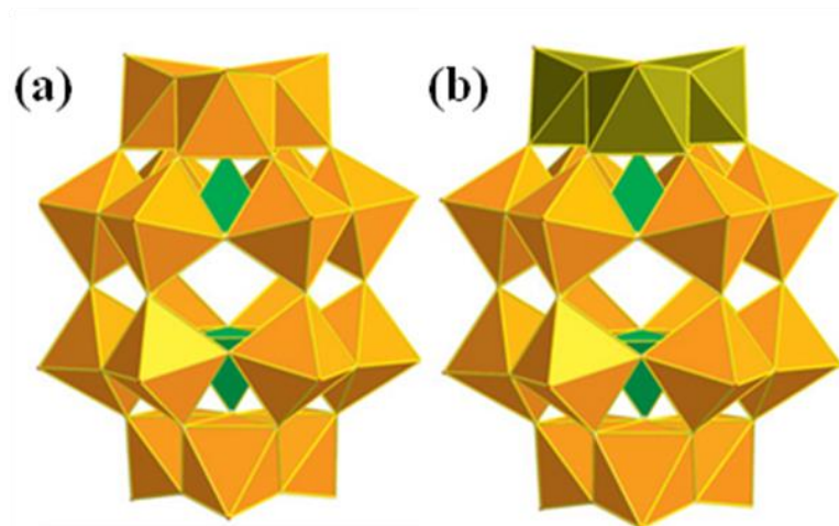
Figure 1.6. Polyhedral representation of the (a) Wells-Dawson anion (b) Trisubstituted Wells-Dawson anion. Color scheme: The gold-colored {MO 6 } octahedra represent the addenda metal, M (Mo, W, V, etc.); the light green {MO 6 } represents the central heteroatom tetrahedron; the dark green {MO 6 } represents the substituted addenda; O, red. 10b
