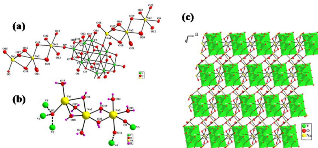
Figure 4. (a) Ball and Stick representation of compound 2 (hydrogen atoms are omitted for clarity); (b) the tri-sodium cation coordinated with the decavanadate anion; (c) 2-D network, established in the coordination polymer of compound 2 , viewed along crystallographic ac plane.
