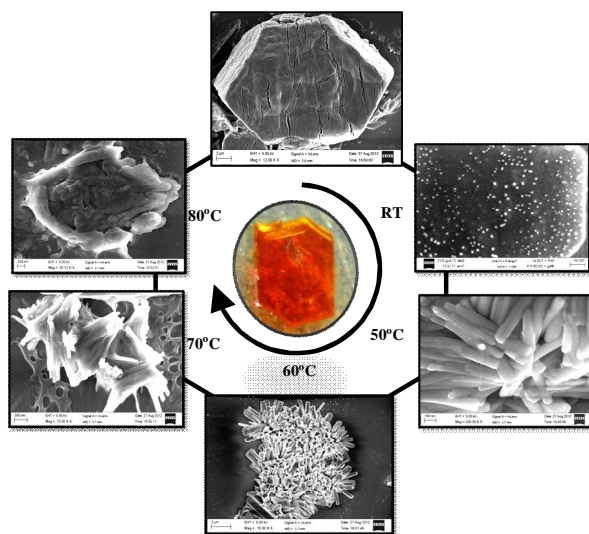
Figure 3. SEM images demonstrating reversible morphological transitions starting from an as-synthesized macro-crystal (at the centre) as a function of sonication temperatures.
