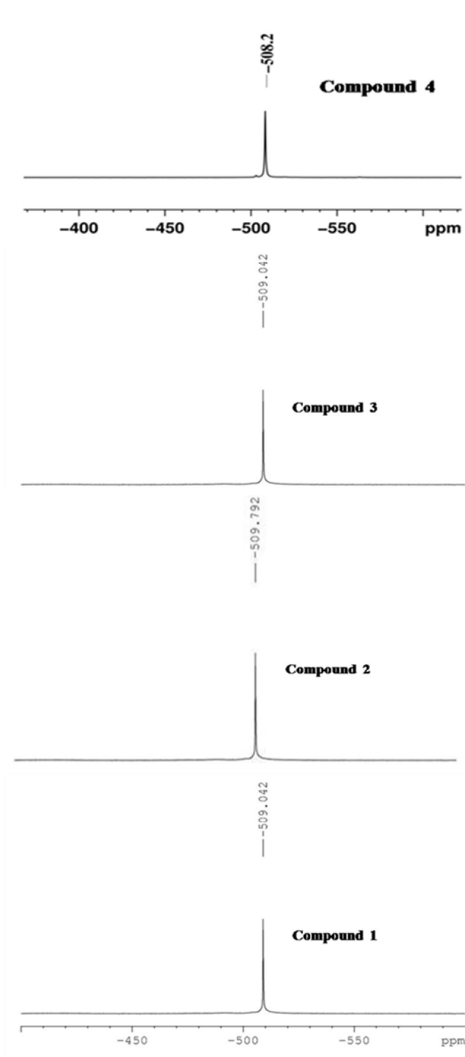
Figure 2.2. ^{51}\text{V} NMR spectra of compounds 1, 2, 3 and 4.
