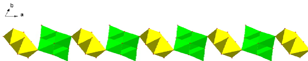
Figure 2.10. Polyhedral representation of 1-dimentional chain viewed along c axis, generated due to coordination of di-sodium aqua-complex cation with cluster anion [V_2W_4O_{19}]^{4-} in compound 3 .
