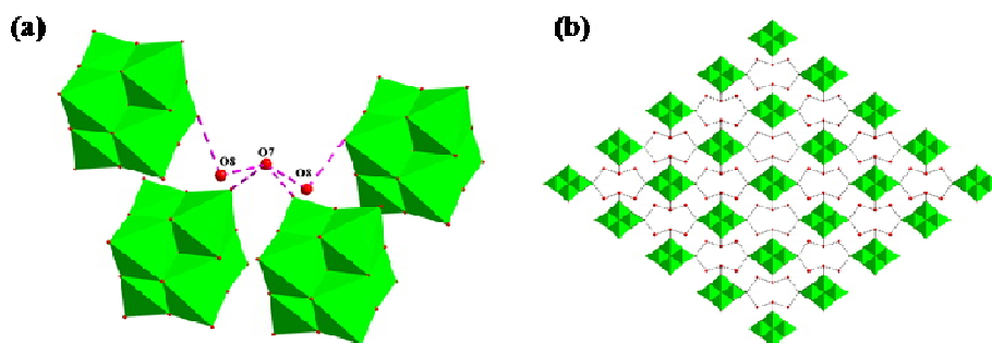
Figure 2.4. (a) A view showing a water trimer connecting four [V 2 W 4 O 19 ] 4+ cluster anions by hydrogen bonds. (b) Three-dimensional supramolecular network, generated due to hydrogen bonding interactions between water trimers and [V 2 W 4 O 19 ] 4+ cluster anions in compound 1 .
