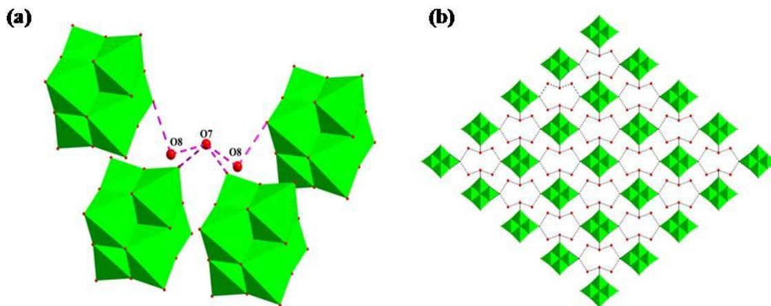
Figure 1. (a) A view showing a water trimer connecting four [\text{V}_2\text{W}_4\text{O}_{19}]^{4-} cluster anions by hydrogen bonds in compound 1 ; (b) three-dimensional supramolecular network, generated due to hydrogen bonding interactions between water trimers and [\text{V}_2\text{W}_4\text{O}_{19}]^{4-} cluster anions in compound 1 .
