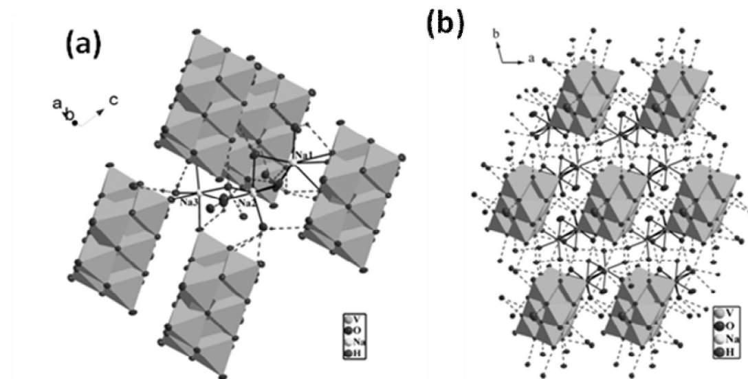
Fig. 4.6. (a) The O–H⋯O interactions between the water molecules of tri-sodium aqua cation with its surrounding five decavanadate anions in compound 2 . (b) The O–H⋯O hydrogen bonding interactions between the anion and cation showing extension from 2D coordination polymer/sheet to a 3D-supramolecular network in compound 2 .
