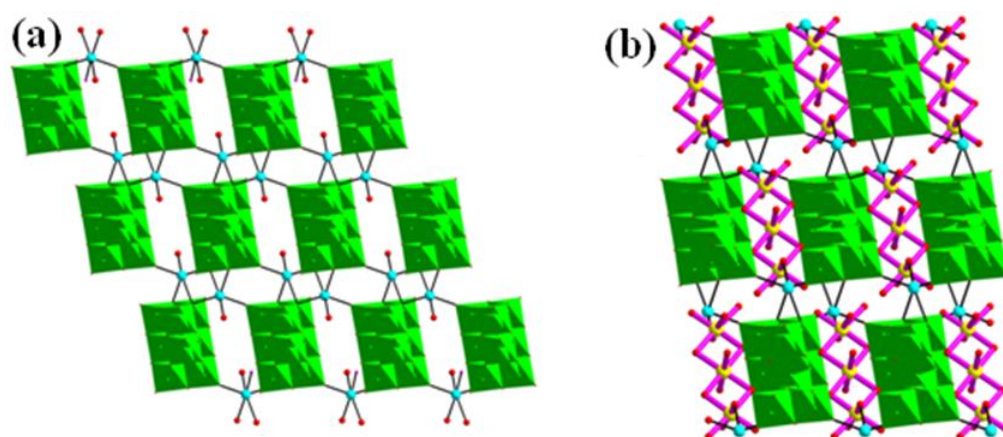
Figure 5. (a) 2-Dimensional layered structure established by the decavanadate cluster anion and silver (I) dimer in the compound 1 along ab plane; (b) 3-Dimensional network established in the polymer of compound 1 due to interlinking of 2-D sheet with the trimeric sodium cation along b -axis.
