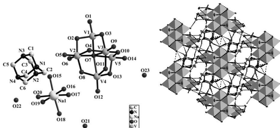
Figure 4.3. Ball and stick representation of the asymmetric unit in the crystal structure of compound 1 (hydrogen atoms are omitted for clarity); (b) 3-d network established due to the O–H \cdots O interactions as well as C–H \cdots O interactions in the compound 1 .
