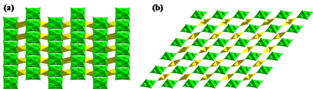
Figure 2. Three-dimensional coordination polymer, formed by linking of sodium-aqua-hexamine coordination complex cation and [\text{V}_2\text{W}_4\text{O}_{19}]^{4-} cluster anion, in the crystal structure of compound 2 : (a) along a axis; (b) along b axis.
