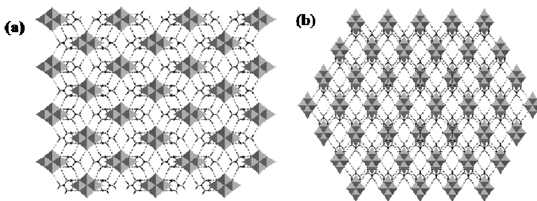
Figure 2.5. Three-dimensional supramolecular network, formed due to C–H...O hydrogen bonding interactions: (a) along crystallographic a axis; (b) along crystallographic b axis.
