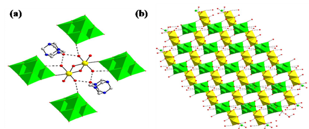
Figure 2.11. (a) The coordination environment of di-sodium aqua-complex with neighboring cluster anions and hexamine in compound 3 ; (b) 3-dimensional frame work established due to O \cdots O interactions in compound 3 .
