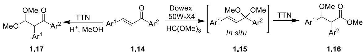
Scheme 1.3: Oxidative rearrangement of chalcones
