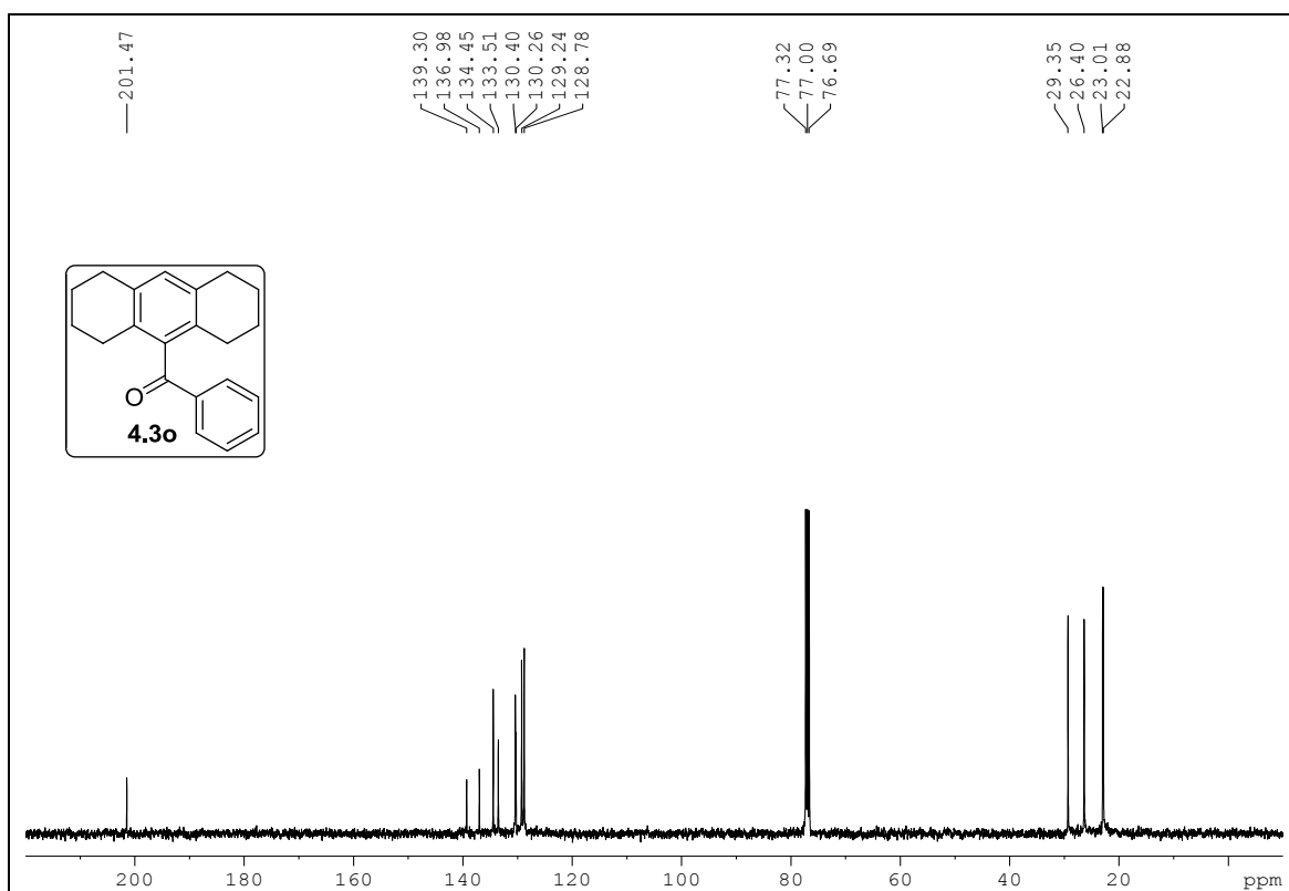
Figure 4.16: ^{13}\text{C} NMR spectrum of compound 4.3o
