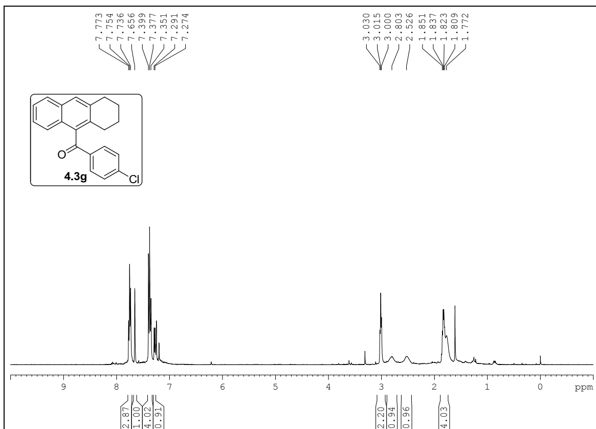
Figure 4.7: ^1\text{H} NMR spectrum of compound 4.3g
