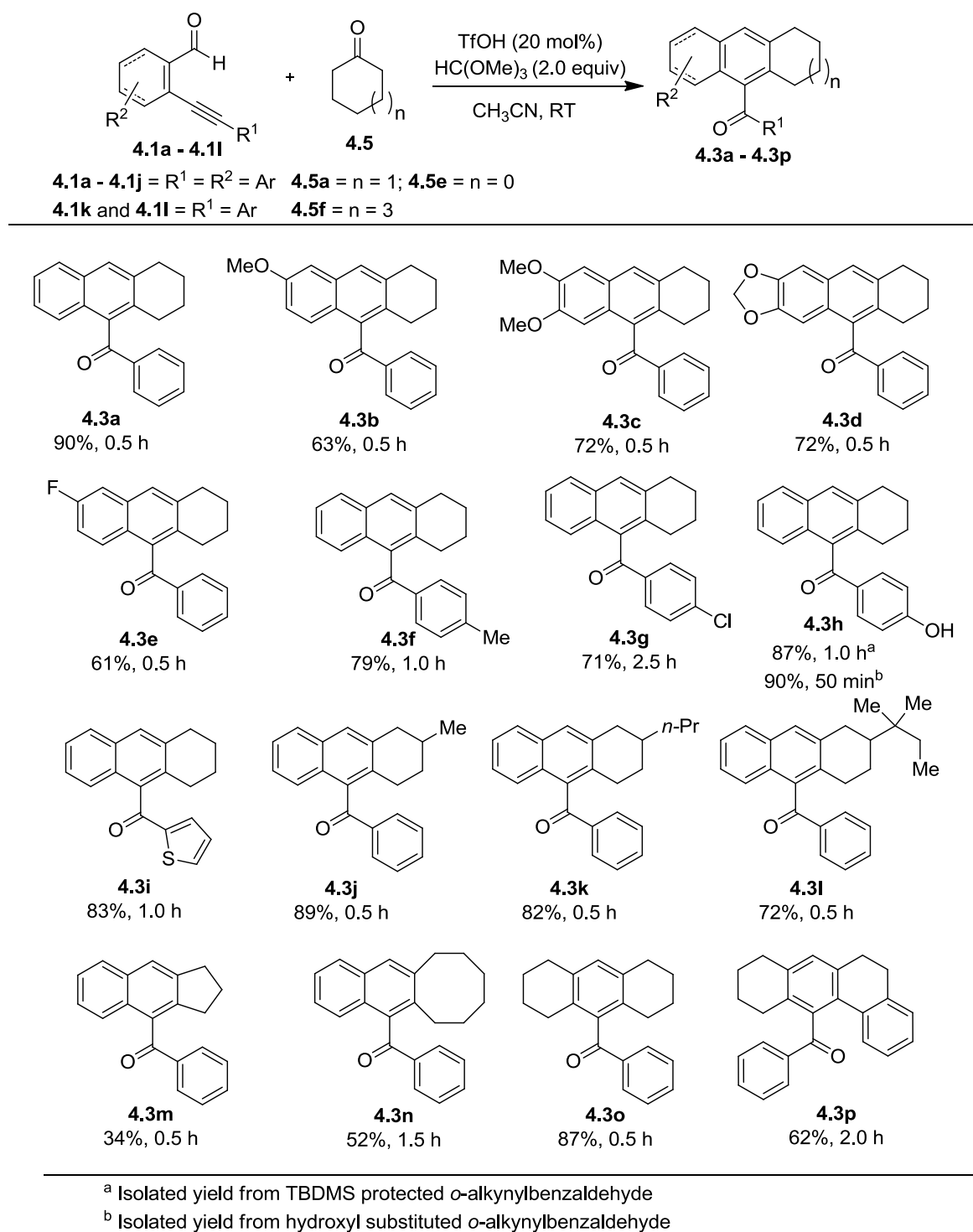
Figure 4.1: Scope of naphthalene formation with cyclic ketones
