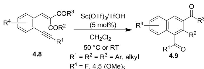
Scheme 4.5: Synthesis of naphthalenes from 2-(2-alkynylarylidenes)-1,3-dicarbonyl compounds
