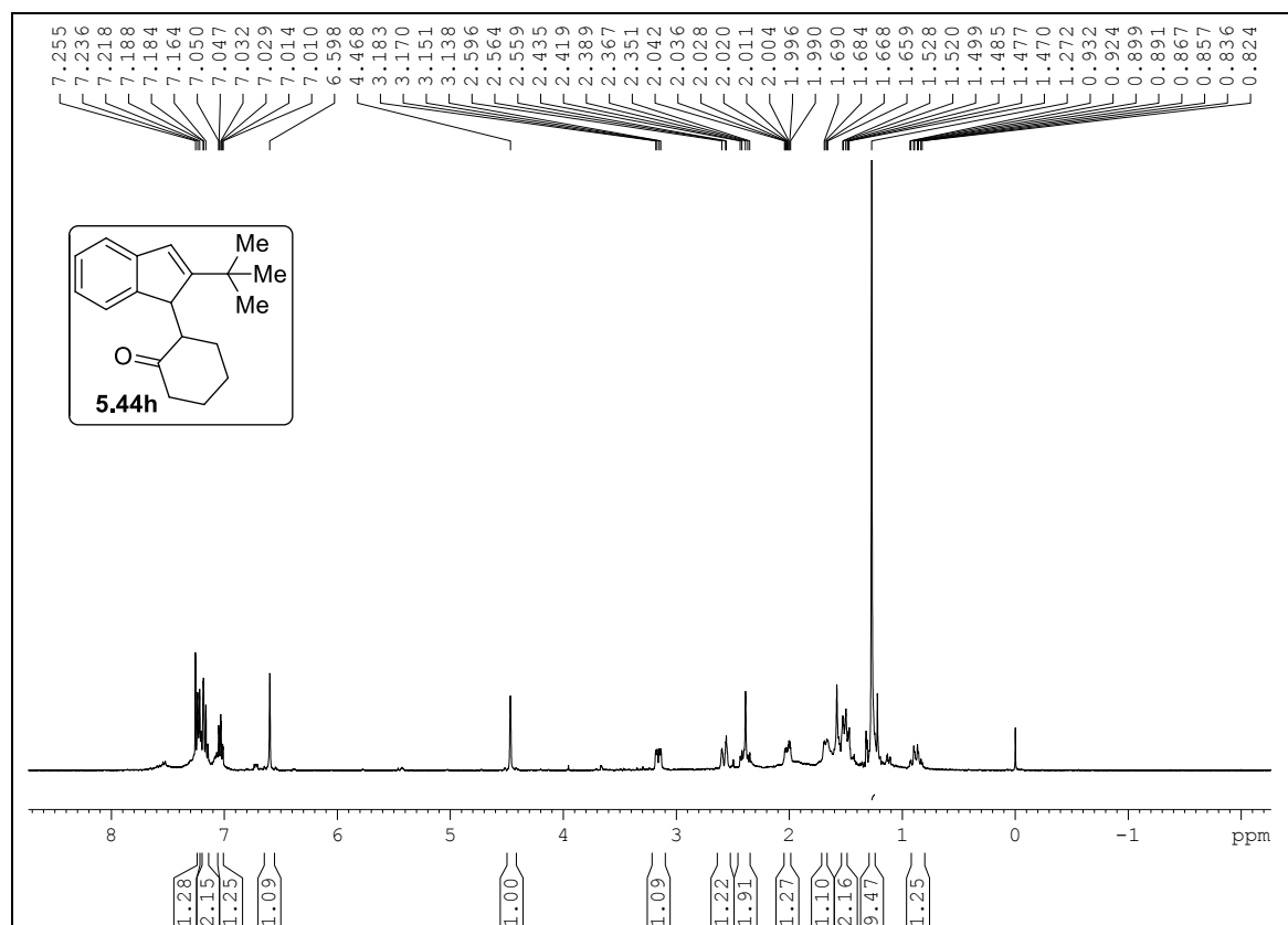
Figure 5.14: 1 H NMR spectrum of compound 5.44h
