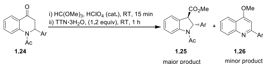
Scheme 1.4b: Oxidative rearrangement of tetrahydro-4-quinolones
