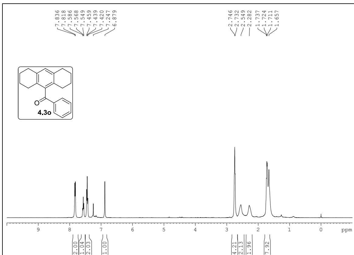
Figure 4.15: ^1\text{H} NMR spectrum of compound 4.3o
