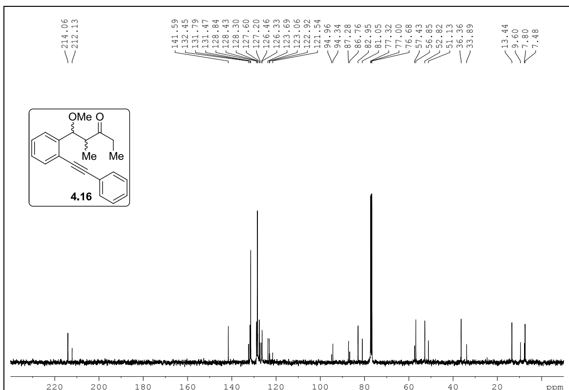
Figure 4.24: 13 C NMR spectrum of compound 4.16
