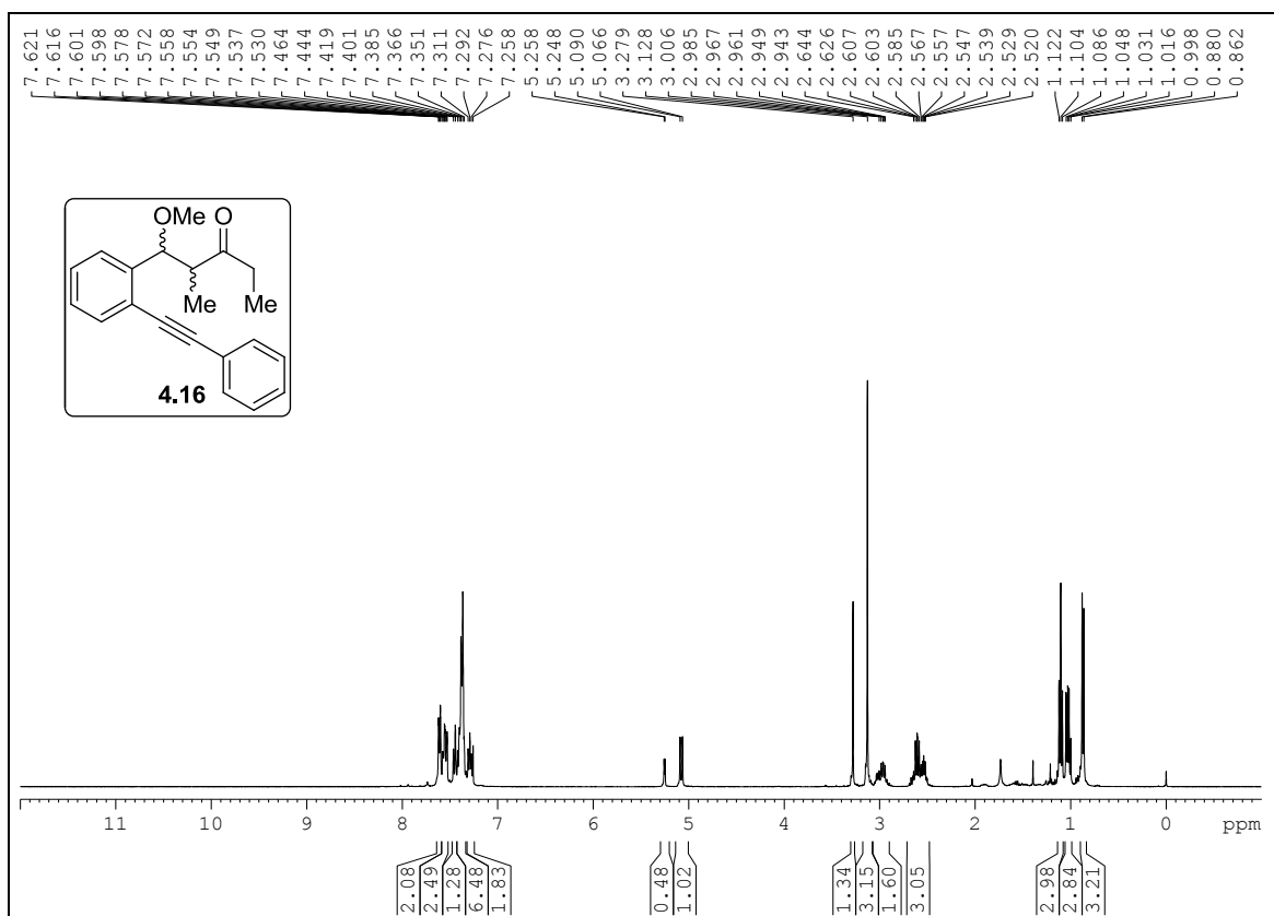
Figure 4.23: 1 H NMR spectrum of compound 4.16
