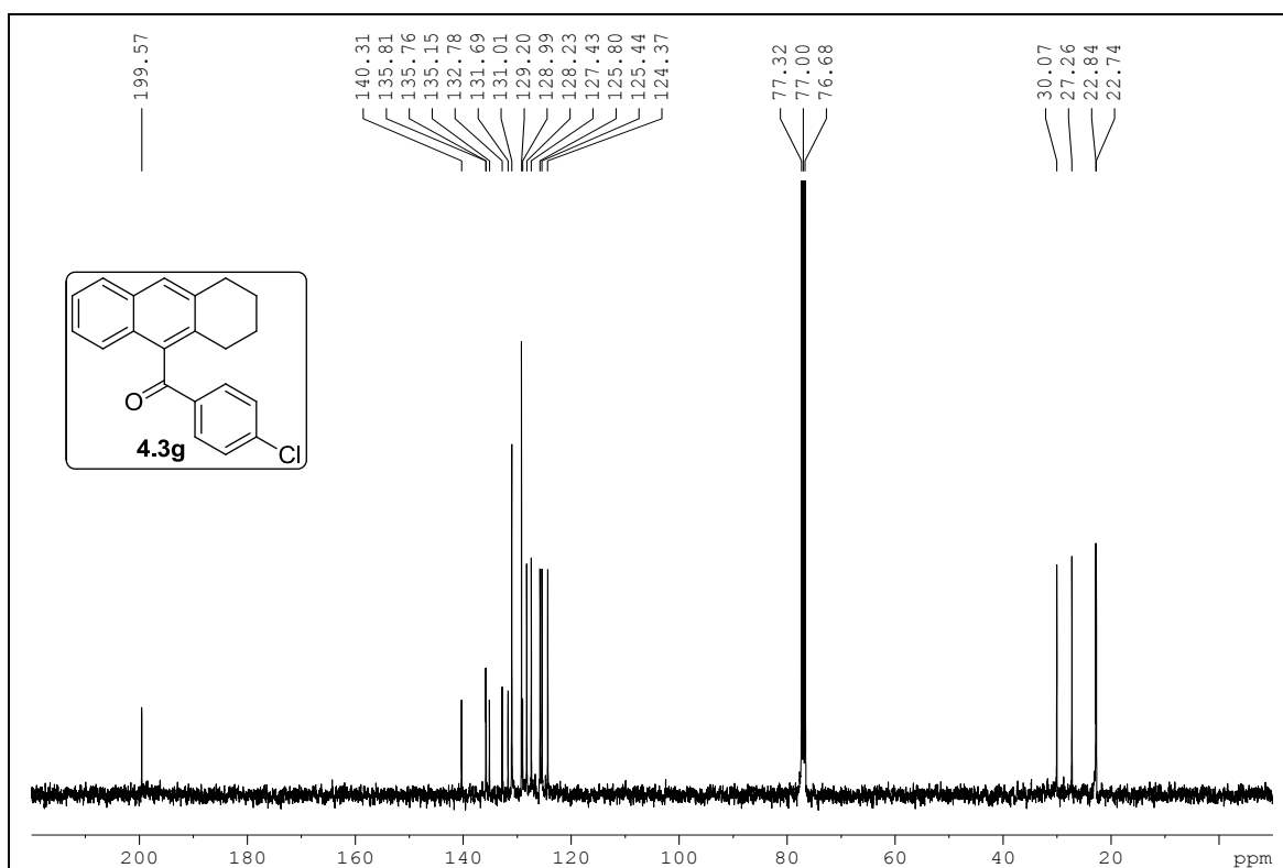
Figure 4.8: ^{13}\text{C} NMR spectrum of compound 4.3g
