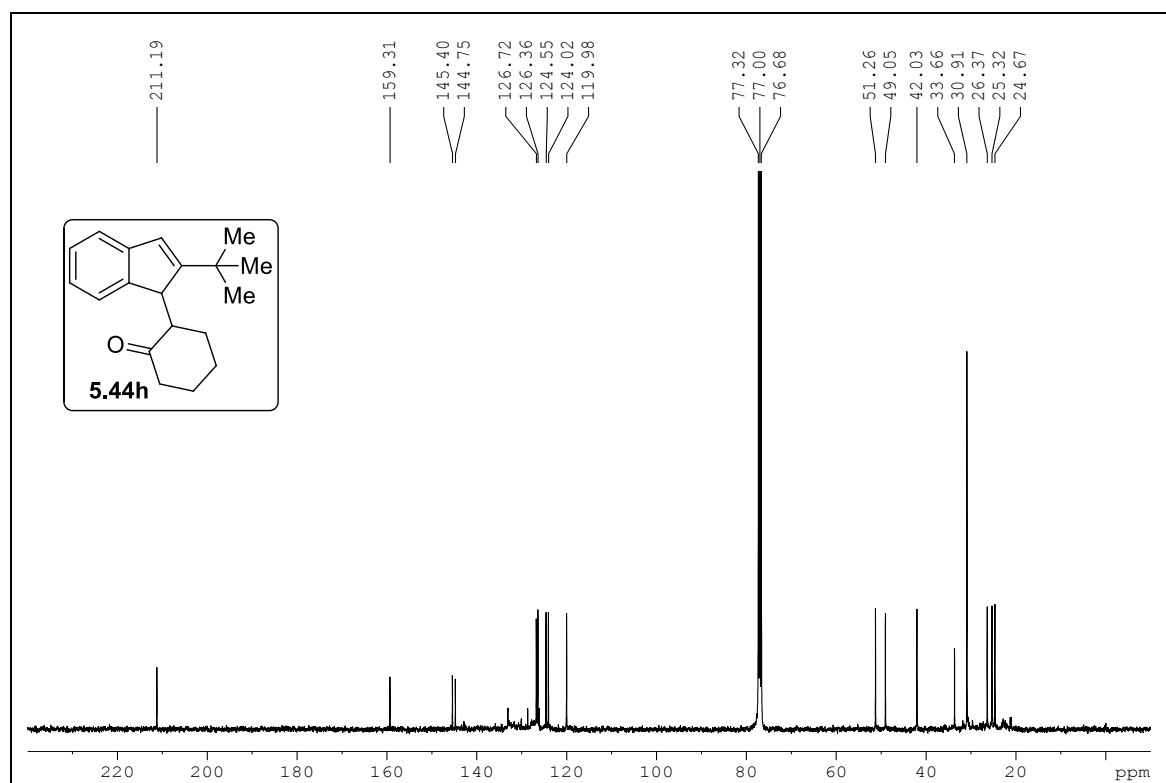
Figure 5.15: 13 C NMR spectrum of compound 5.44h
