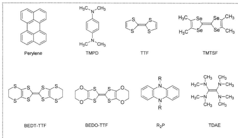
Figure 1.8 Molecular structures of \pi -electron donors.
