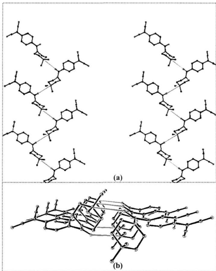
Figure 3.14 M -helical assembly in 19.H 2 O crystal along the b axis; the electrostatic interactions (cyan) are indicated between O10 and N17 for easier viewing : (a) stereo view perpendicular to the helical axis and (b) view along the helical axis. C (black), N (blue) and O (red) atoms are shown.
