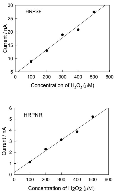
Figure 3.11: Calibration plot between \text{H}_2\text{O}_2 concentration and current response for HRP coupled with Safranin O (HRPSF) and HRP coupled with Neutral red (HRPNR). Linear response to the concentration of hydrogen peroxide is observed upto 500 \mu\text{M} concentration.
