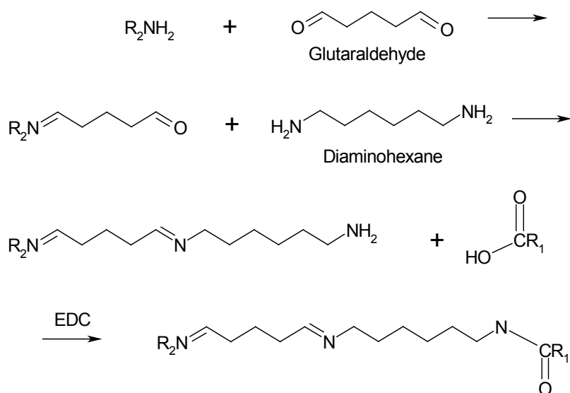
Figure 3.3: Covalent coupling of the dyes ( R_2NH_2 ) to the carboxylic groups present in the acidic residues of HRP ( R_1COOH ) with a spacer arm diamino hexane using glutaraldehyde and EDC.
