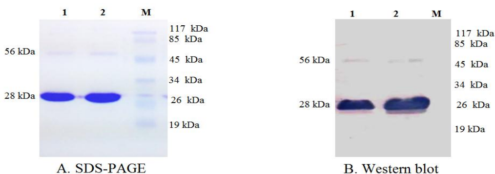
Fig 3.6: SDS-PAGE and western blots analysis of TSV (Sunflower strain) purified virus. In Panel A, Lane 1 and 2: TSV purified virus, M: protein ladder. Left side of the SDS-PAGE gel indicates purified virus molecular weight as 28 kDa and 56 kDa. Right side of the gel indicates molecular weight of marker. In panel B, Lane 1 and 2: TSV purified protein, M: protein ladder. Left side of the western blot indicates antisera reacted with the purified virus at 28 kDa and 56 kDa. Right side of the blot indicates molecular weight of marker
