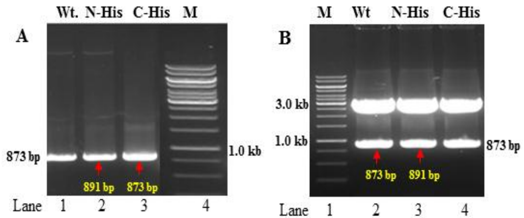
Fig 6.4 PCR amplification and cloning of three versions of MP; wild type, N-terminus histag and C- terminus histag
