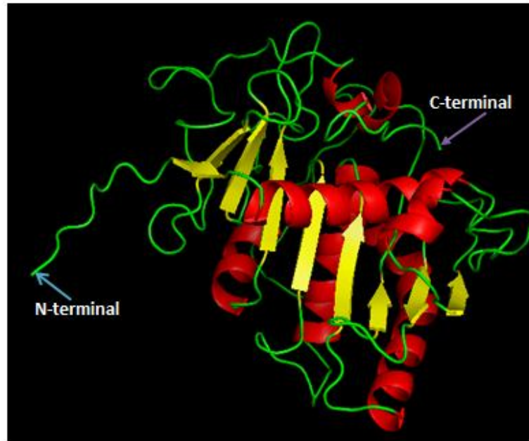
Fig 6.12: 3-Dimensional homology model of TSV movement protein.
