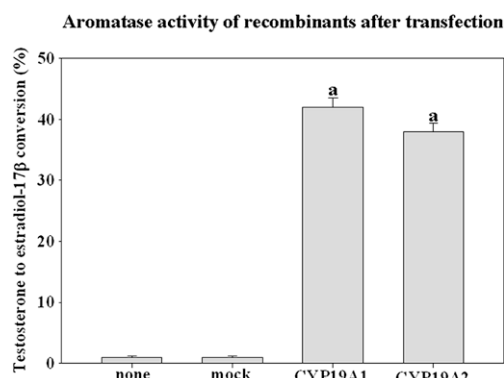
Fig. 2. Representative histogram showing the % conversion of testosterone to estradiol-17β by CYP19A1 and CYP19A2 recombinant protein. Common letters indicate means that are not significantly different ( P < 0.05 ).
