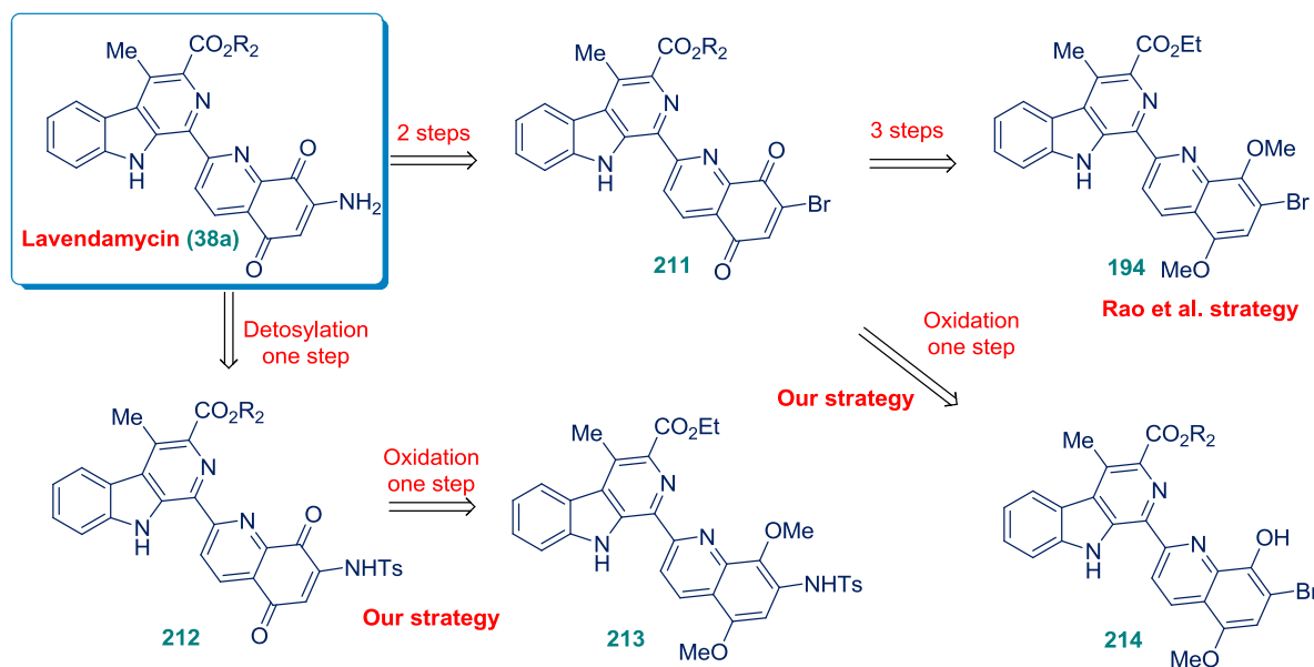
Scheme 16
