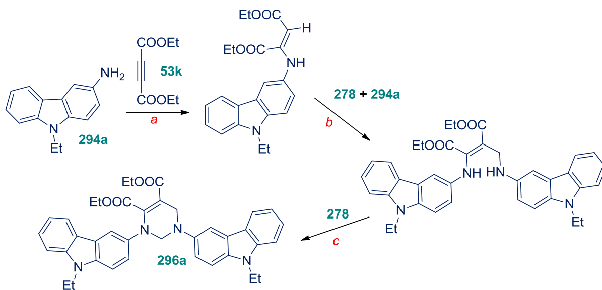
Scheme 39
