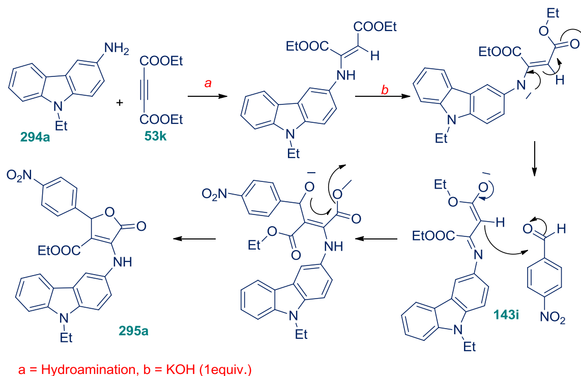
Scheme 37
