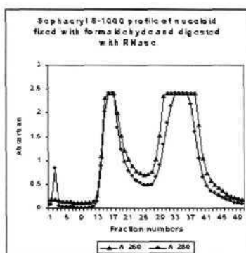
Fig 13a: Sephacryl S-1000 column elution profile of Sulfolobus acidocaldarius nucleoid fixed with formaldehyde at exponential phase and digested with RNase.
