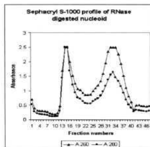
Fig 11a: Sephacryl S-1000 column elution profile of Sulfolobus acidocaldarius nucleoid isolated from cells at exponential phase and digested with RNase.
