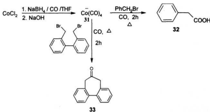
Scheme 9
