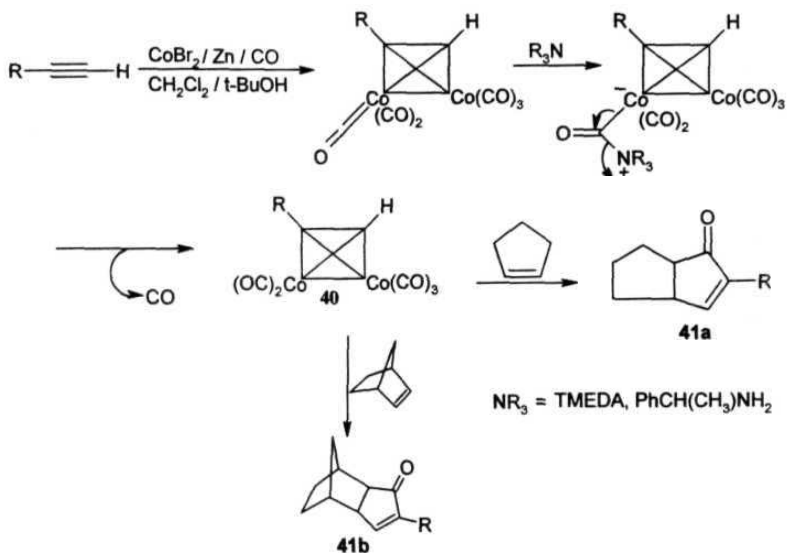
Scheme 7
