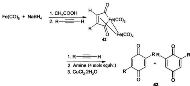
Scheme 8
