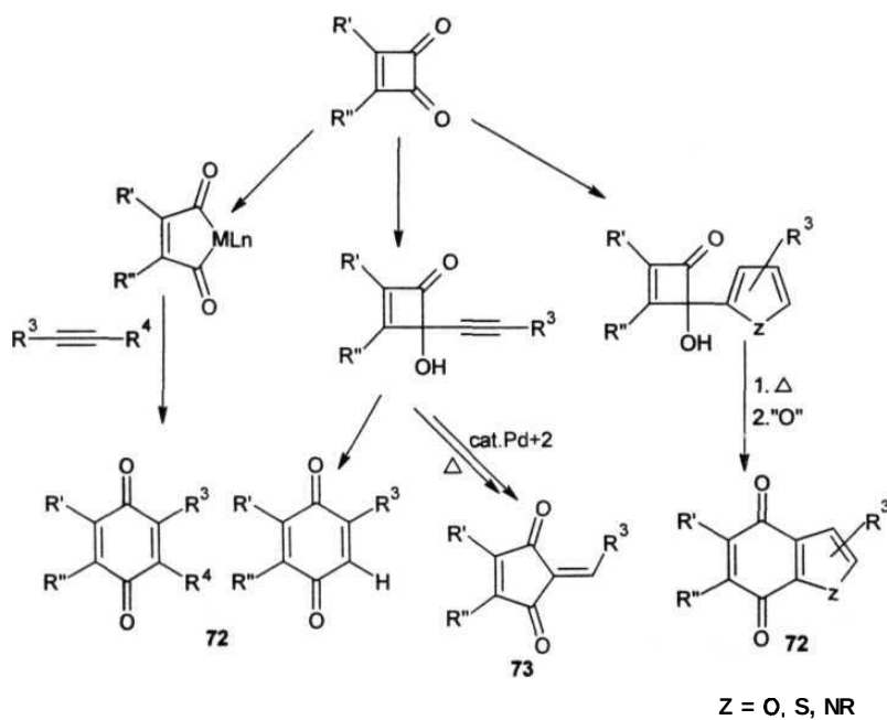
Scheme 16
