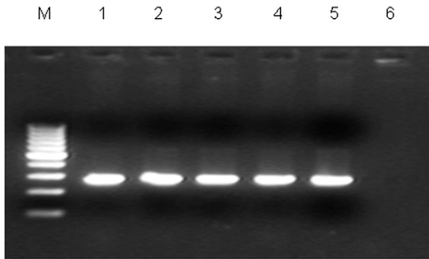
Figure 2. PCR based detection of O25b subgroup that is linked to the B2-O25b-ST131-CTX-M-15 clonal group of strains. Among 32 ESBL producers in our collection ( n = 150 ) four were positive for O25b subgroup (Lanes 1 to 4); lane 5, positive (strain showing consistently positive); lane 6, negative; M, 100 bp DNA ladder. doi:10.1371/journal.pone.0018063.g002
