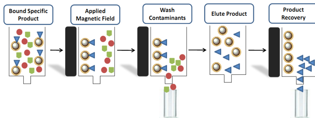
Figure.1.6. Schematic representation of a bio separation process using MNPs as adsorbent.
