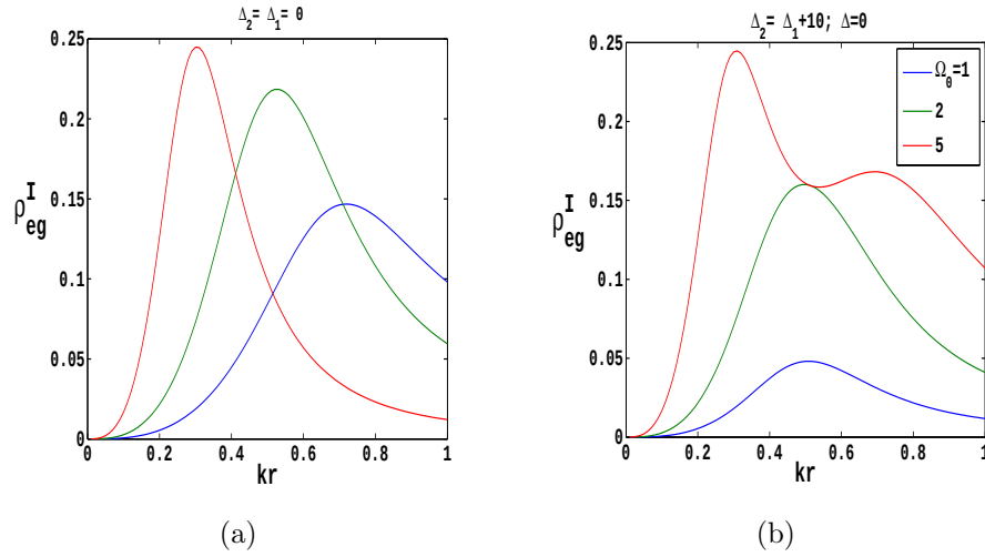
Figure 2-12: The atomic coherence Im(\rho_{eg}) on resonance for 2-12(a) identical atoms 2-12(b) non-identical atoms.
