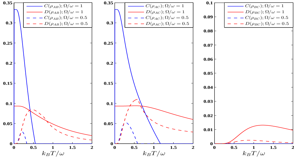
Figure 4-10: Loop configuration: Pairwise C(\rho_{ij}) and D(\rho_{ij}) as a function of k_B T / \omega for different values of \Omega/\omega = 1, 0.5 .
